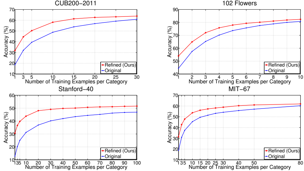
Figure 3.6: Model type evaluation between models learned from few samples and models refined by our model regression network on these four benchmark datasets. We evaluate the logistic regression as the model of interest. The robust performance shows generic transformations for different types of models.
