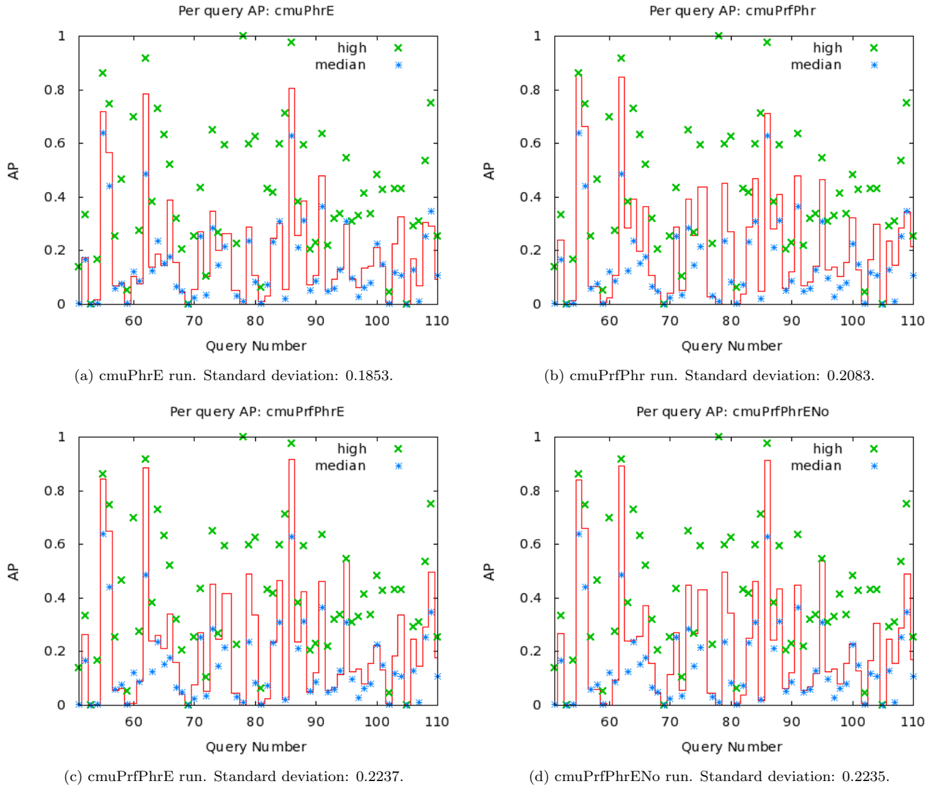
Figure 4: Per query analysis of AP values for all relevant tweets on TREC 2012 dataset.
