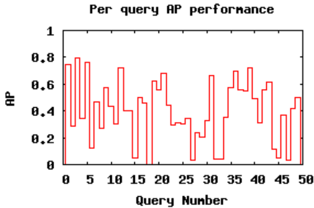
(c) Phrase run. Standard deviation: 0.2206
