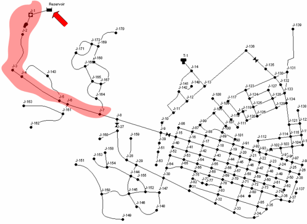
Figure 5: Water distribution network: Sensor 1-7 are highlighted since they are close to reservoir (red arrow) and on the main pipe.
