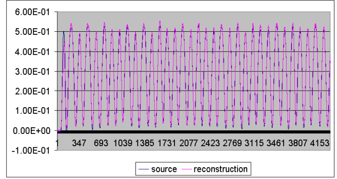
Figure 2: Chlorine reconstruction; reconstruction based on 2 hidden variables are very close to the original value.
