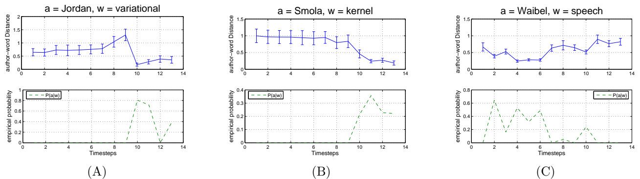
Figure 5. Average distance between author-word pairs over time (above), along with corresponding empirical probabilities (below). A. Jordan and variational. B. Smola and kernel. C. Waibel and speech. The graphs on the bottom reflect empirical \bar{p}(\text{author} | \text{word}) from the NIPS data which varies inversely over time with the average author-word distance in the embedding shown in the top row, demonstrating the responsiveness of the embeddings to the underlying data.
