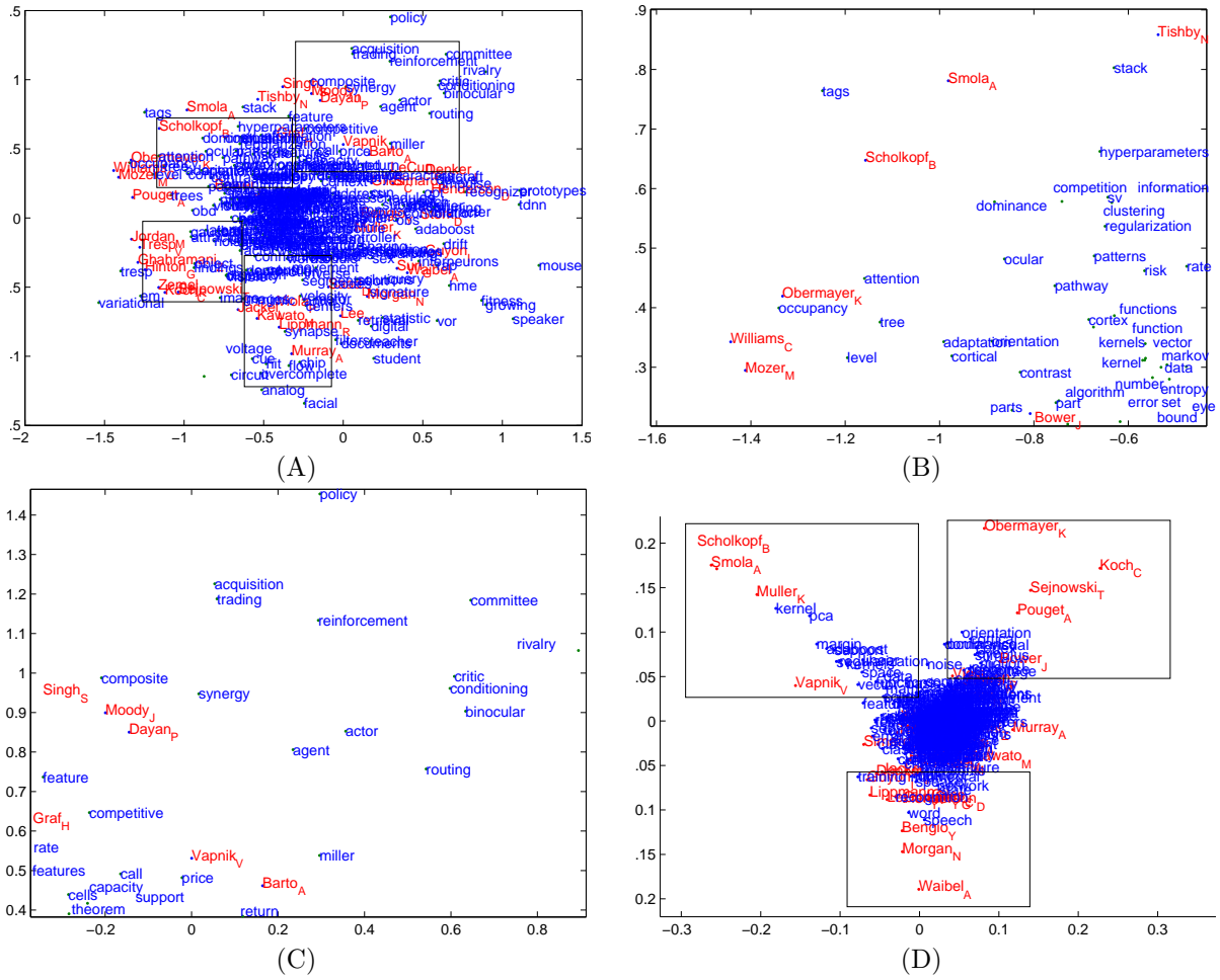
Figure 4. (A). t = 13 Dynamic embedding of NIPS data (final timestep, 1999). (B),(C). Close-ups of (roughly) the top two rectangles in (A). The first Both contain authors and keyword groups that are interrelated (e.g. (B) contains entities related to kernels, (C) contains reinforcement-learning-related terms and authots. (D). PCA embedding of aggregate counts matrix of NIPS data, that averages out any sequential patterns.
