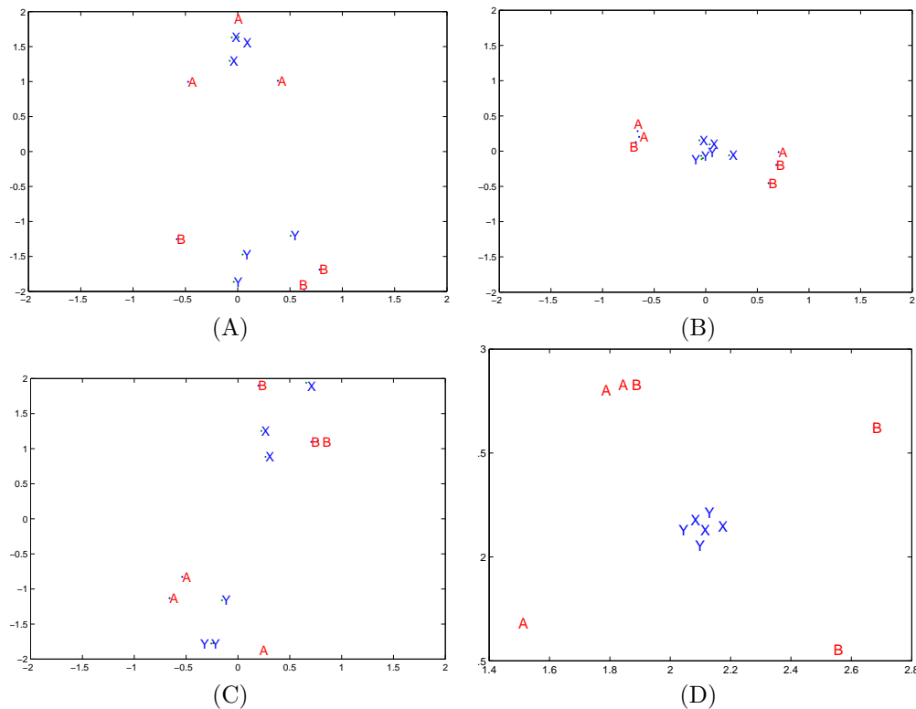
Figure 3. Dynamic embedding of synthetic data vs. static embedding. A, B are two groups of authors and X, Y are two groups of words. The 140-timestep data smoothly varies from strong A - X and B - Y links to strong A - Y and B - X links. The entities are initialized randomly (not shown). A. t = 20 , strong A - X and B - Y links. B. t = 70 , Intermediate configuration, noisy uniform links. C. Strong A - Y and B - X links. D. A static embedding of the aggregate co-occurrence matrix, which is effectively a noisy uniform matrix, resulting in entities mixing with each other.
