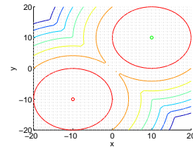
Figure 2. A plot of the log normalizing constant \log(e^{-(x-a)^2-(y-b)^2} + e^{-(x-c)^2-(y-d)^2}) for two given coordinates a, b and c, d . Two things are apparent: the correlation of x and y coordinates, and the presence of multiple optima in this function. We desire an approximation that preserves the x - y correlation.
