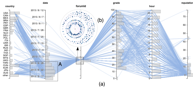
Figure 5: Filtering posts in Study Groups , with (a) being the Feature Statistics View, and (b) the corresponding network graph.
