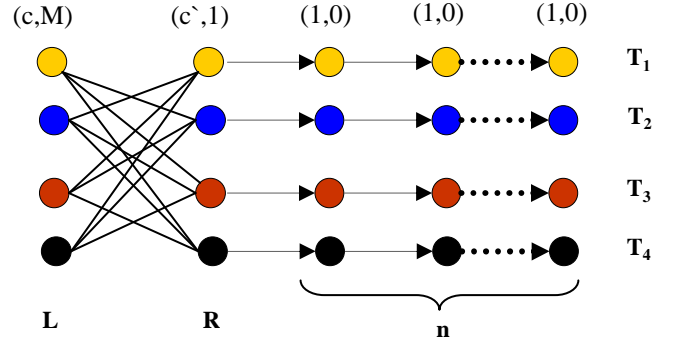
Figure 2: An illustration of a bidding problem with a large integrality gap ( k = 3 ).
