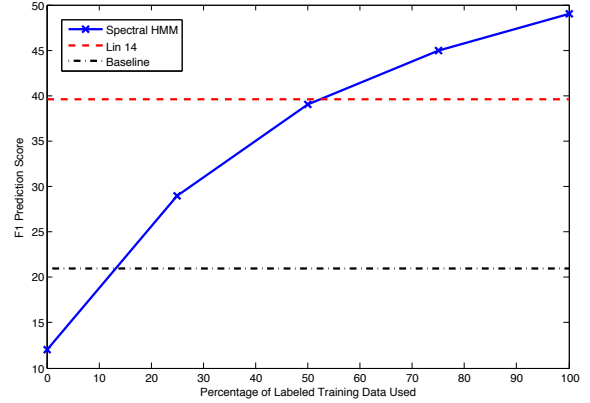
Figure 2: Empirical results for labeling of implicit relations.
