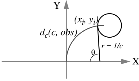
Figure 1: Obstacle Distance Calculations
