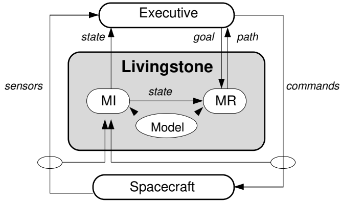
Fig. 1. Livingstone mode identification (MI) and mode recovery (MR)
