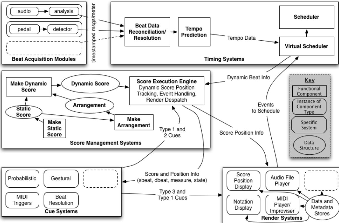
Figure 1: A Reference Architecture for HCMP
