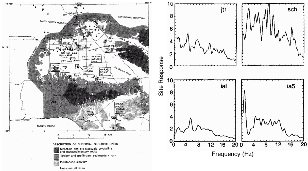
Figure 8. (a) Location of sites in SFV instrumented for studying spatial variation of ground motion of 1994 Northridge earthq. aftershock; (b) spectral ratios at indicated locations derived from recorded seismograms (Hartzell et al, 1996).
