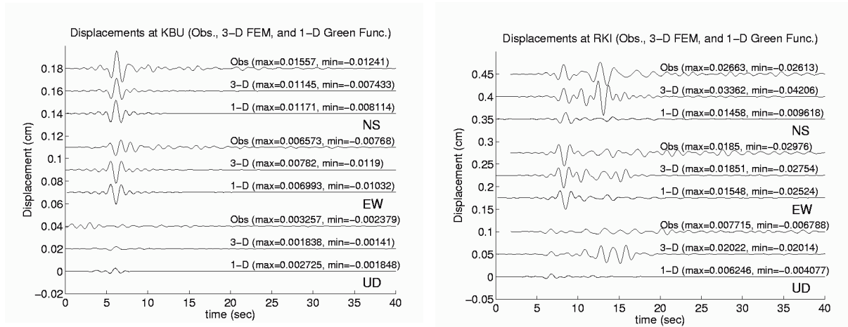
Figure 7. (a) Band-passed displacements (0.9-5.0 s) observed and simulated for a 1995 Kobe earthq. aftershock at sites KBU and RKI (see Fig. 10a) (Hisada et al, 1998).
