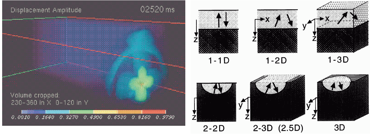
Figure 1. (a) Instantaneous displacement pattern in San Fernando Valley (from Quake animation, www.cs.cmu.edu/~quake ; (b) Dimensionality of problems used for studies of site effects (Hisada and Yamamoto, 1996)
