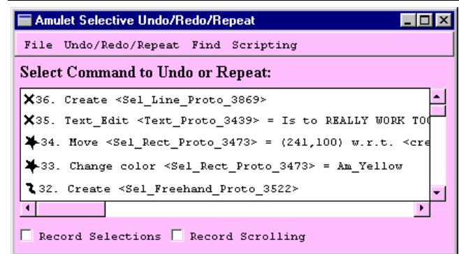
Figure 9. Undo dialog box [13] for PebblesDraw where each command is marked with the shape for the user who performed it.
