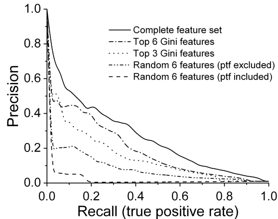
Figure 2. The average precision vs. recall curve of the Random Forest model trained on the complete feature set, in comparison to models trained with a subset of features. The top 3 Gini features are degree, betweenness centrality, and GO neighbor process similarity features. The top 6 Gini features are the top 3 Gini features plus clustering coefficient, GO neighbor function, and location features. These are compared to two baseline classifiers, where 6 features are randomly selected from the set of features that does not include the top 6 Gini features, with and without protein type features (ptf).
