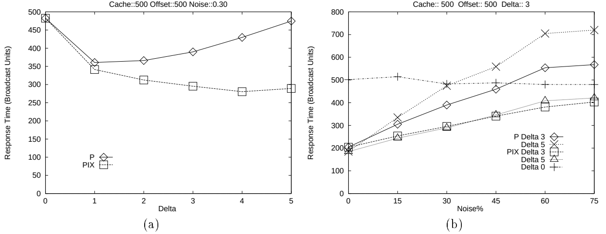
Figure 9: \mathcal{P} vs. PIX with (a) varying \Delta (b) varying noise
