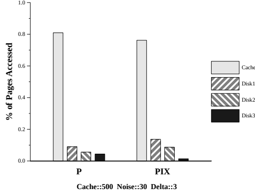
Figure 10: Access Locations for \mathcal{P} vs. PIX for 30% noise
