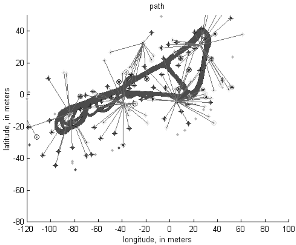
Figure 12 Constellation map and vehicle trajectory. Five constellations were formed by the algorithm. The intersection of the bases are presented with a '+' and the other side of the segment with a 'o'. The relative landmarks are represented with '*' and its association with a base is represented with a line joining the landmark with the origin of the relative coordinate system
