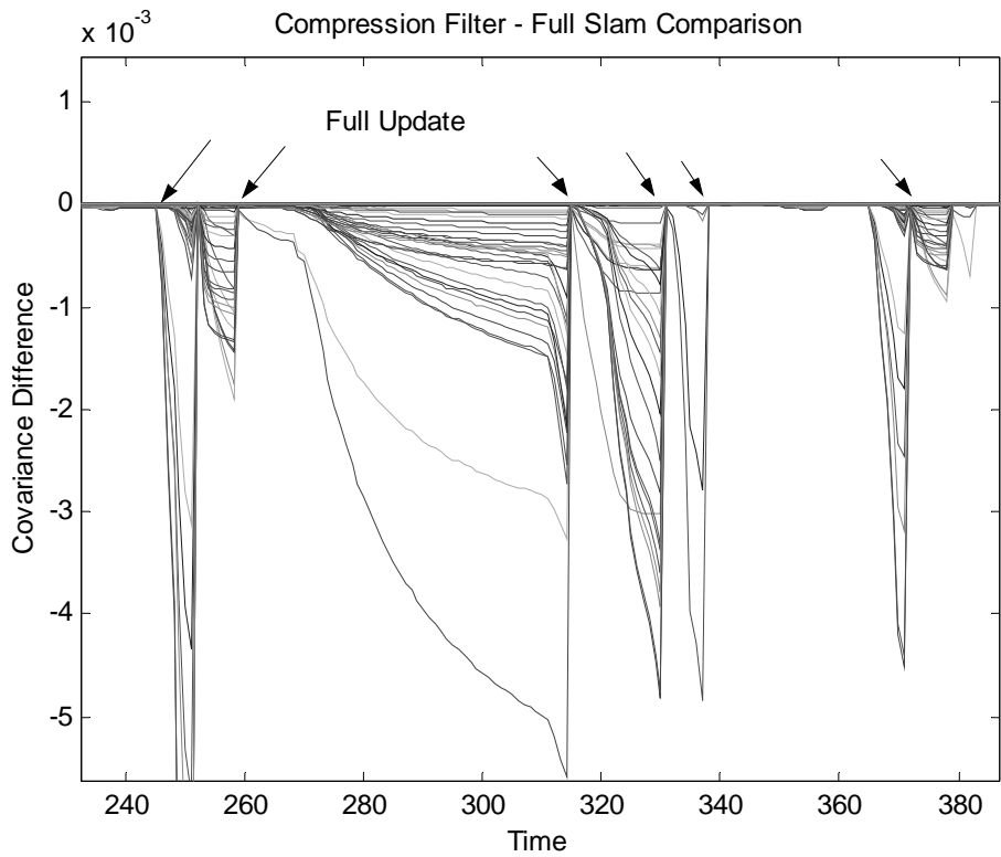
Figure 16 Estimated error differences between full slam and compressed filter. The estimated error difference between both algorithms becomes identically zero when the full update is performed by the compressed algorithm.
