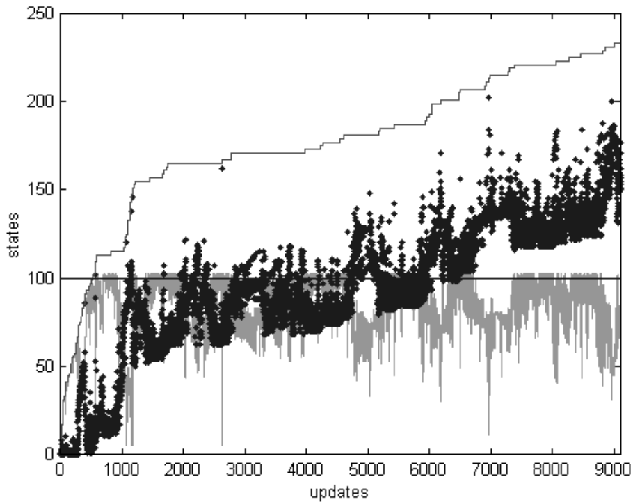
Figure 18 Total number of states and states used and not updated. In this run a maximum number of states was fixed as constraint for the sub-optimal SLAM algorithm. This is appreciated in the grey plot where the maximum number of states remain below a given threshold. The number of states not updated increases with time.
