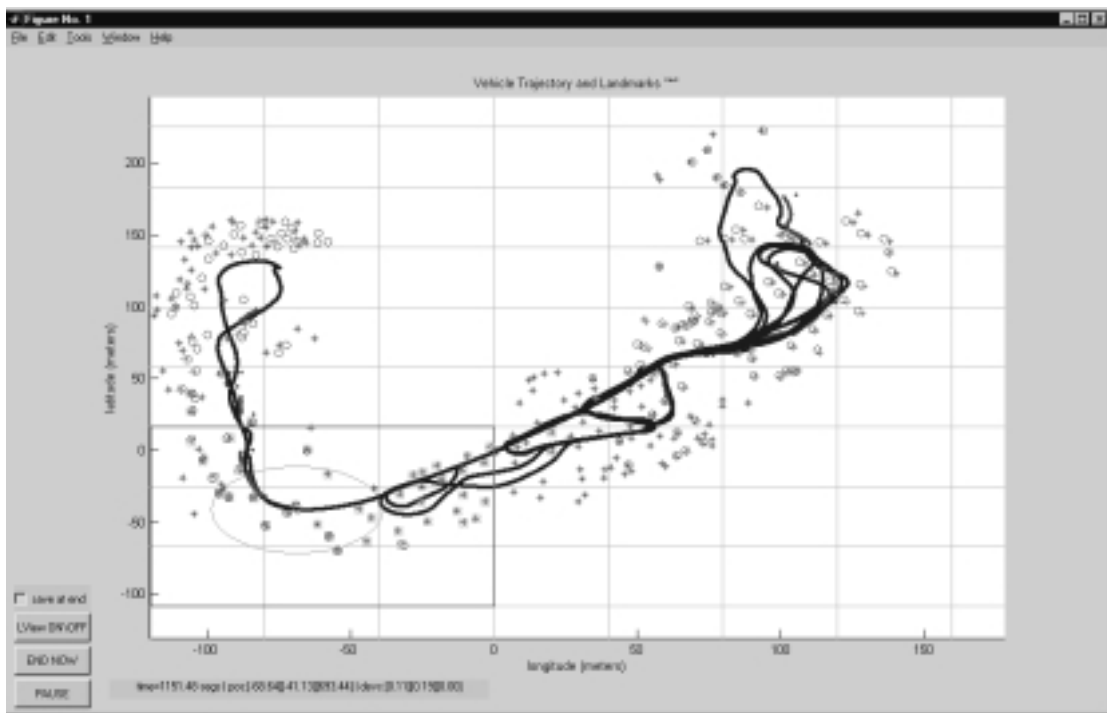
Figure 13 Vehicle and local areas. This plot presents the estimated trajectory and navigation landmark estimated position. It also shows the local region 'r' with its surrounding regions. The local states X_A are the ones included in the nine regions shown enclosed by a rectangle in the left button corner of the figure.
