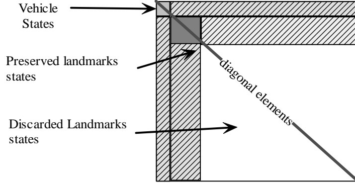
Figure 4 Full covariance matrix divided into the covariance blocks corresponding to the Vehicle and Preserved landmarks states ( X_P ) and Discarded landmarks states ( X_D ). The cross-correlation covariance between the Preserved and Discarded states are fully updated as shown in grey. Finally the cross-correlation between the elements of the states corresponding to the “Discarded landmarks” are not updated as shown in white.
