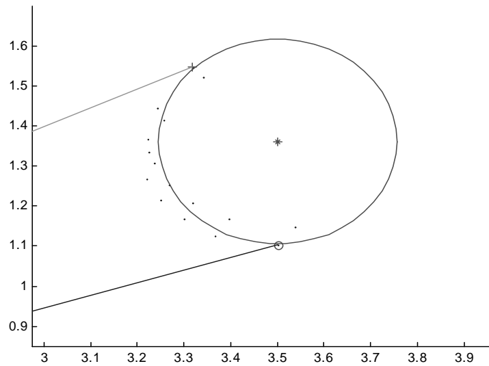
Figure 8 Tree profile and system approximation. The dots indicate the laser range and bearing returns. The filter estimates the radius of the circumference that approximates the trunk of the tree and centre position.
