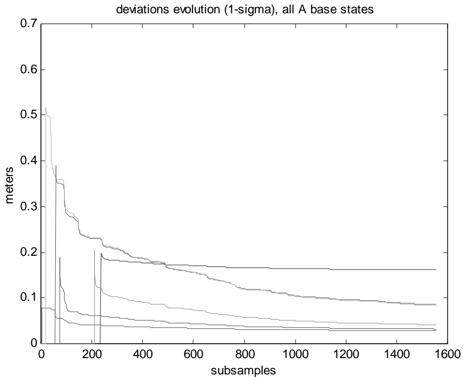
Figure 21 estimated error history of the bases using most of the states.
