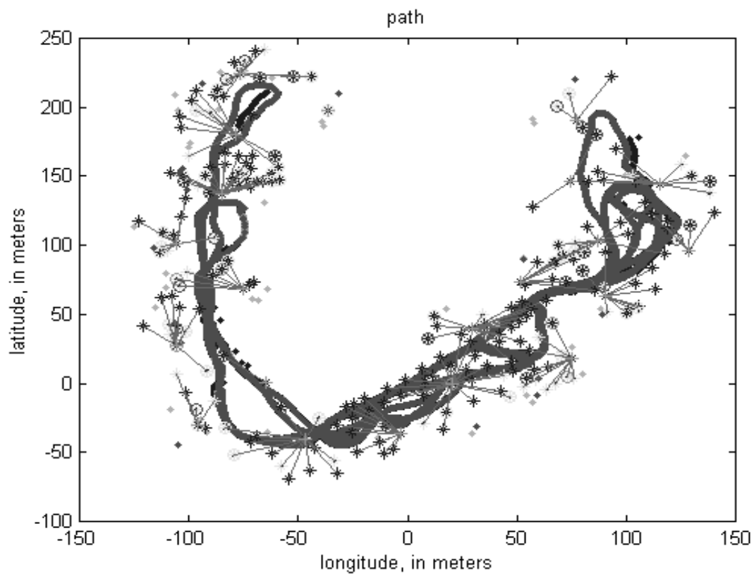
Figure 25 Long trajectory with Compressed SLAM. This plots present a run in a very large area that demonstrates the benefits of the compressed algorithm. In this case 18 constellations were created.
