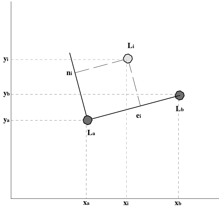
Figure 5 Local reference frame. The reference frame is formed with two landmarks. The observation are then obtained relative to this frame.
