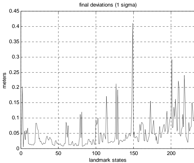
Figure 19 final estimation errors for relative and absolute states using most of the states.
