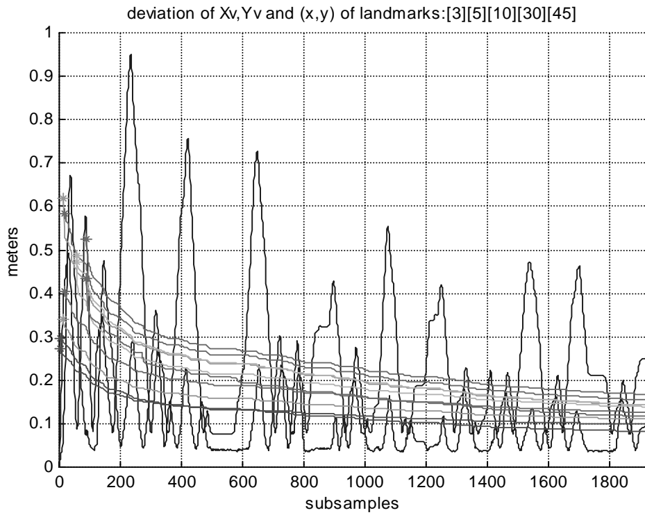
Figure 10 History of selected state's estimated errors. The vehicle states shows oscillatory behaviour with error magnitude that is decreasing with time due to the learning of the environment. The landmarks always present a exponential decreasing estimated error with a limit of the initial uncertainty of the vehicle position.
