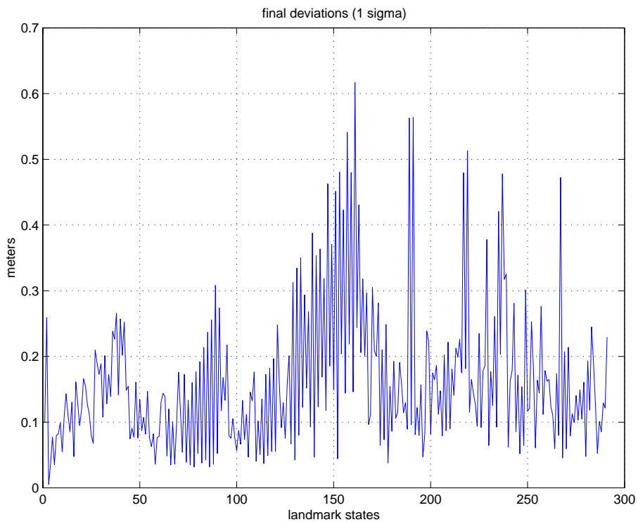
Figure 11 Final estimated error of all states. For each state the final estimated error is presented. The maximum error is approximately 60 cm.
