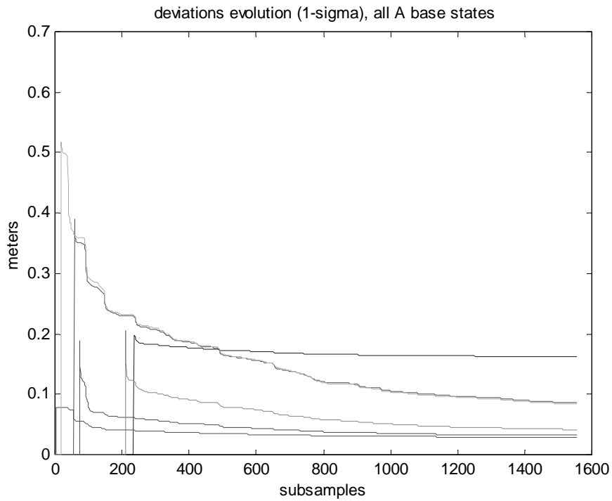
Figure 22 Estimated error history of the bases with reduced number of states
