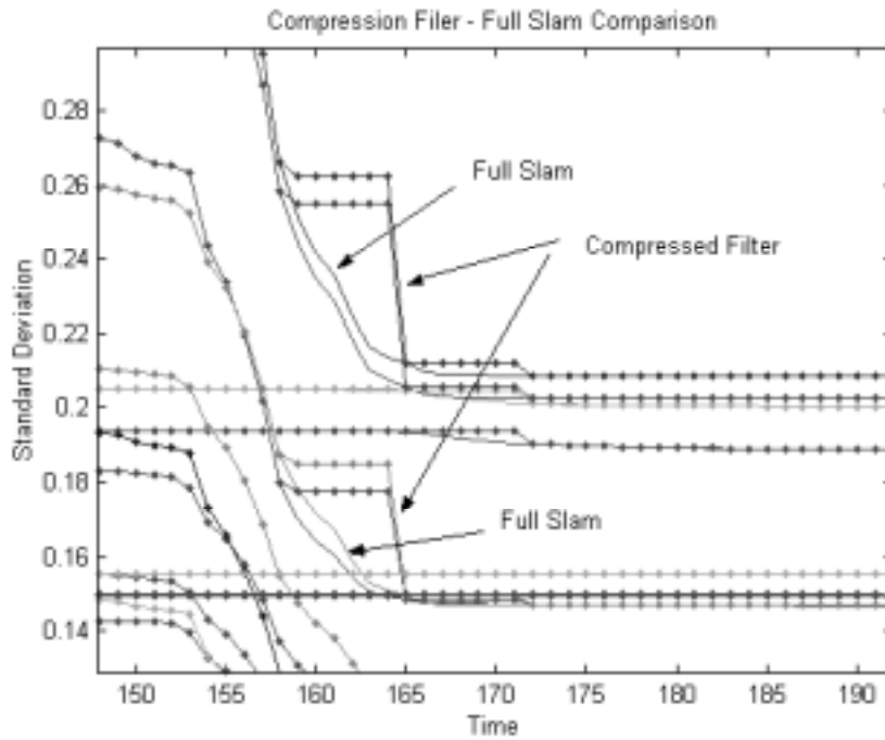
Figure 14 Landmark estimated position error for full Slam and compressed filter. The solid line shows the estimated error provided by the full SLAM algorithm. This algorithm updates all the landmarks with each observation. The dotted line shows the estimated error provided by the compressed filter. The landmark that are not in the local area are only updated when the vehicle leaves the local area. At this time a full updates is performed and the estimated error becomes exactly equal to full SLAM
