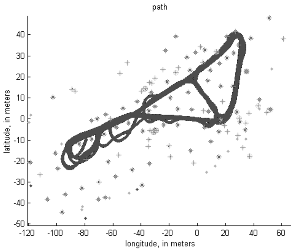
Figure 9 Vehicle trajectory and landmarks. The '*' shows the estimated position of objects that qualified as landmarks for the navigation system. The dots are laser returns that are not stable enough to qualify as landmarks. The solid line shows the 20 minutes vehicle trajectory estimation using full SLAM.
