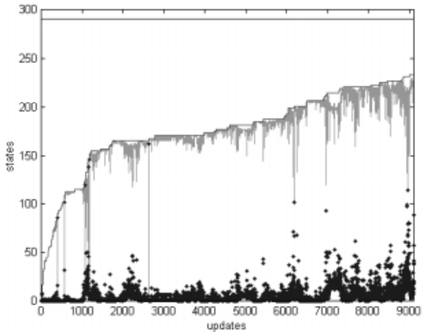
Figure 17 Total number of states and states used and not updated. The figure presents the total number of states with a solid black line. This number is increasing because the vehicle is exploring new areas and validating new landmarks. The states used by the system are represented in grey. The number of states not used is represented with '*'. In this run the system used most of the states available.
