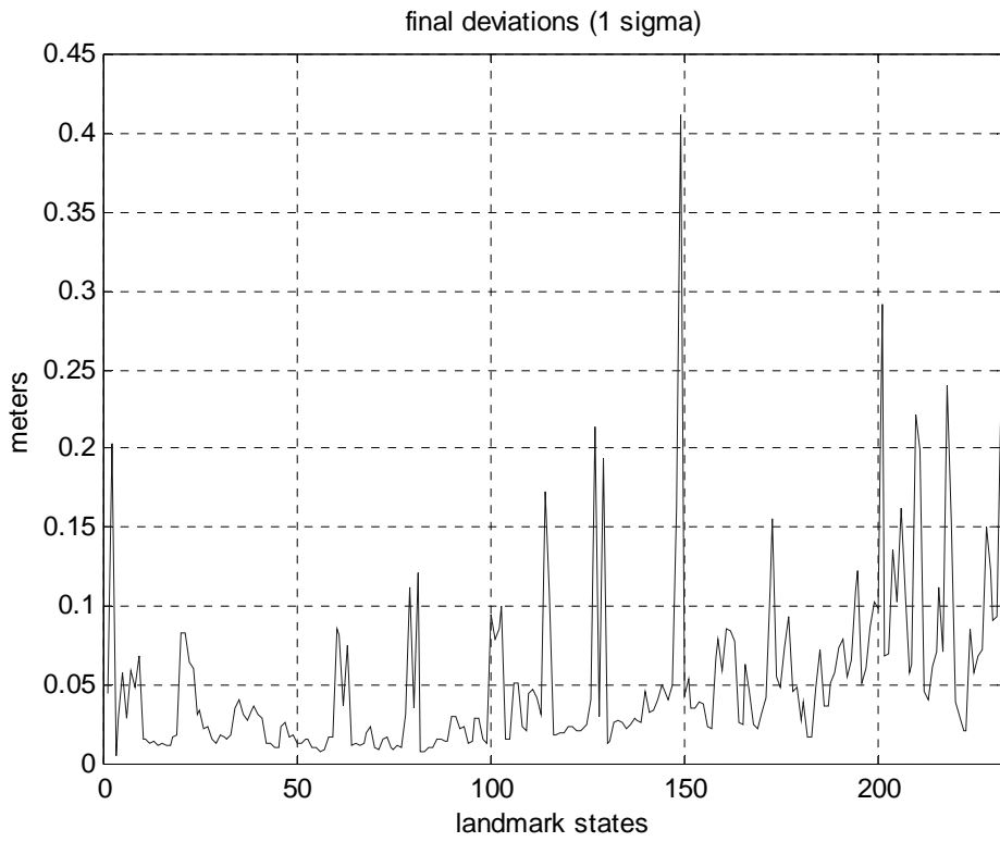
Figure 20 Final estimated error of relative and absolute states using a reduced number of states. These results are similar to the ones using most of the states. This result shows that the proposed algorithm is not only consistent but close to optimal when used with the appropriate map representation.
