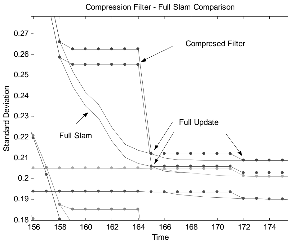
Figure 15 Landmark estimated position error for full Slam and compressed filter (enhanced). This plot present a cleared view the instant when the compressed algorithm performed a full update. A this time (165) the full slam (solid line) and the compressed algorithm (solid lines with dotes) report same estimated error as predicted.
