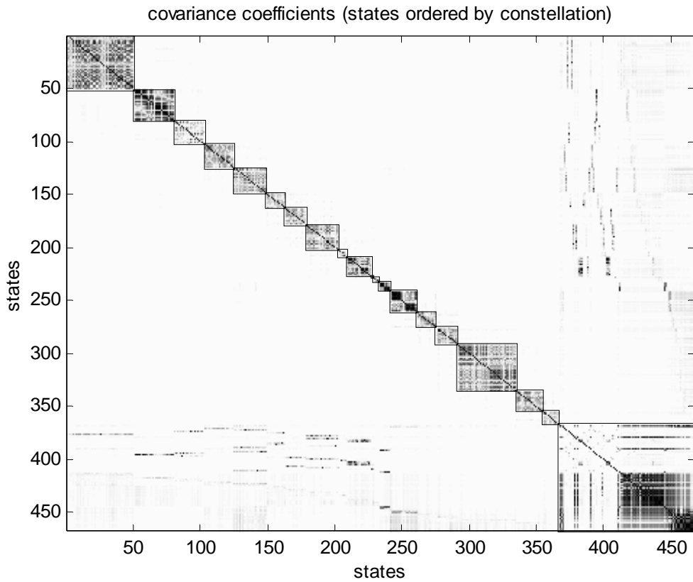
Figure 26 Cross correlation coefficients. The plots shows 18 constellation and a block in the right hand corner containing the correlation coefficient for the bases and the vehicle states. It can be appreciated that the crosscorrelation between the relative states of the different bases is very small.
