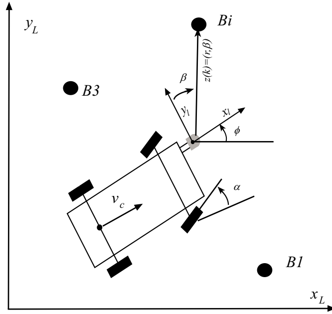
Figure 1 Vehicle coordinate system
