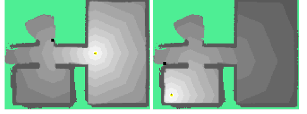
Figure 6: Target positions obtained using the coordination approach. In this case the target point for the second robot is to the left in the corridor.
