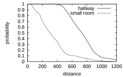
Figure 5: Probability P(d) of measuring at least d given the histograms in Figure 3 and 4.
