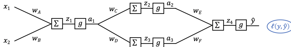
Figure 5: Neural Network
