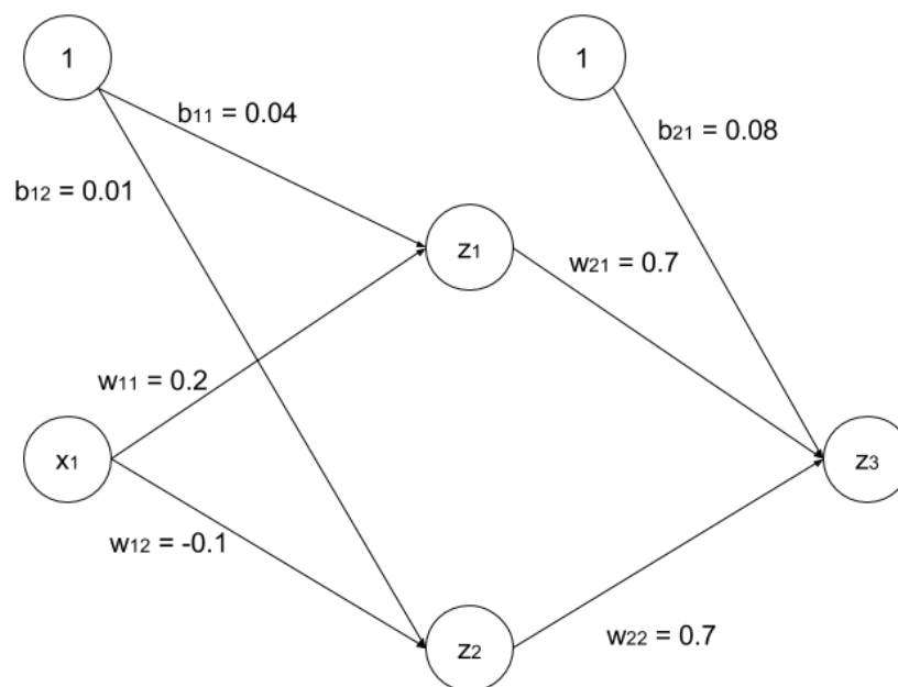
Figure 1: Neural Network
