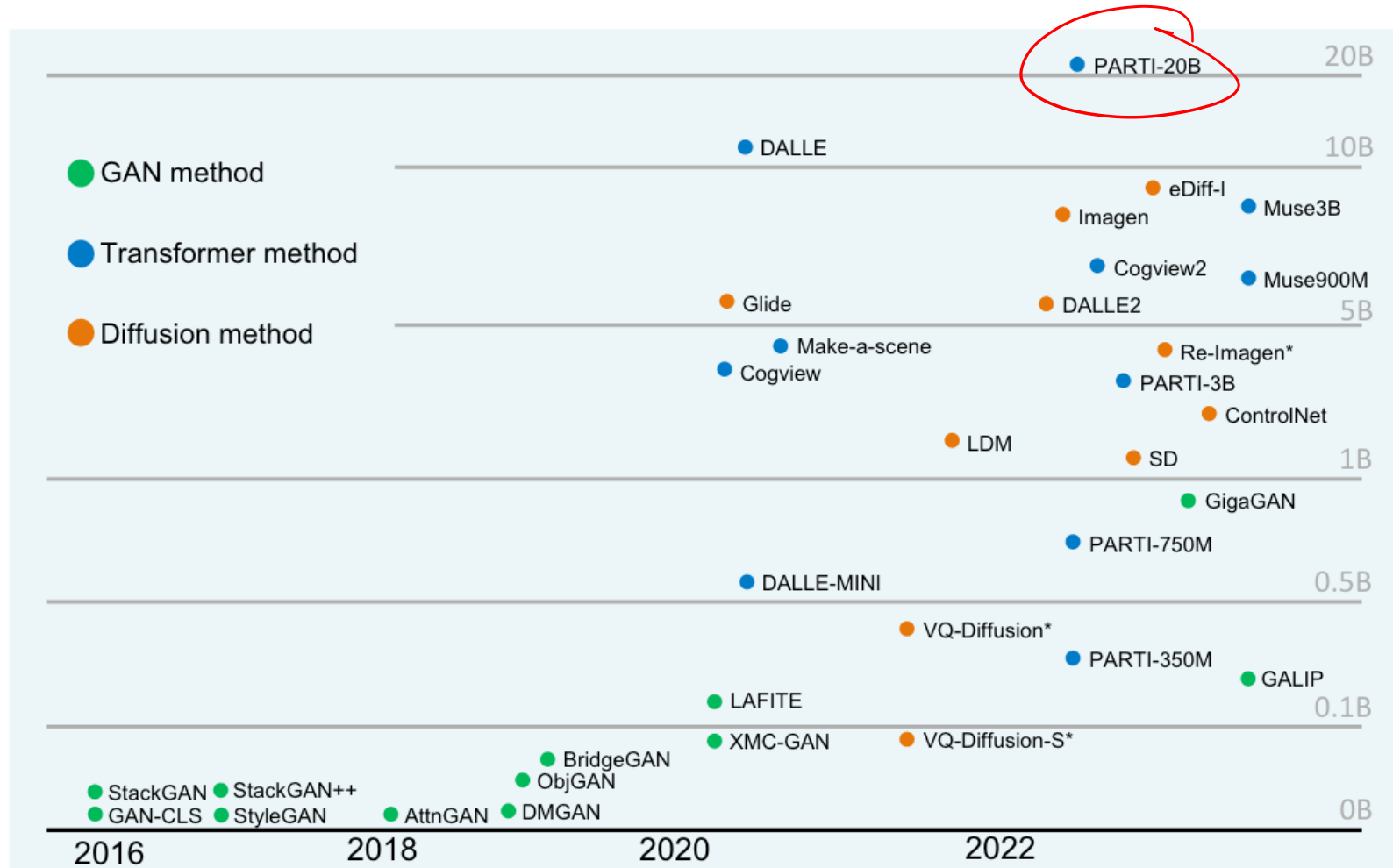
Fig. 5. Timeline of TTI model development, where green dots are GAN TTI models, blue dots are autoregressive Transformers and orange dots are Diffusion TTI models. Models are separated by their parameter, which are in general counted for all their components. Models with asterisk are calculated without the involvement of their text encoders.
