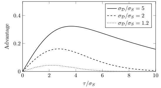
Fig. 1: The advantage of Adversary 4 as a function of t ’s influence \tau . Here t is assumed to be binary and uniformly distributed.
