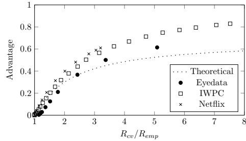
(b) Regression and tree models assuming knowledge only of \sigma_S .
