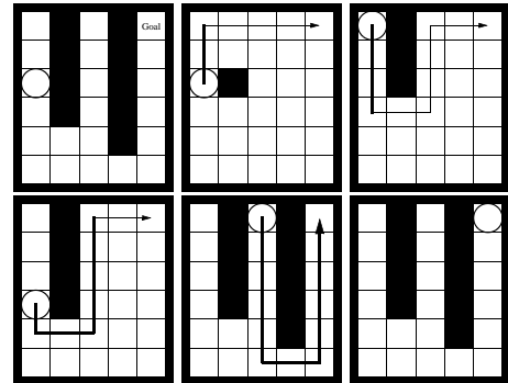
Figure 1: Planning with the Freespace Assumption: The goal cell is in the upper-right corner. The upper-left figure shows the terrain. The circle denotes the game character, and black cells denote blocked cells. The remaining figures show the knowledge that the game character has about the terrain at various points in time. The circle again denotes the game character, black cells denote blocked cells that the game character has already observed, the line denotes the cost-minimal presumed unblocked path from the current cell of the game character to the goal cell, and the thick part of the line denotes the beginning of the path that the game character actually traverses until it reaches the goal cell or observes the path to be blocked (and re-plans).
