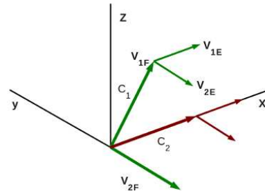
Fig. 5: Same RPY, different arm configurations.
