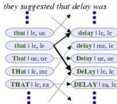
Figure 1: Given individual histories, the decodings delay and DeLay , are most probable - perhaps in the context of “time delay” and respectively “Senator Tom DeLay”
