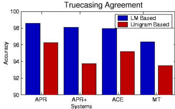
Figure 3: LM truecaser vs. unigram baseline.
