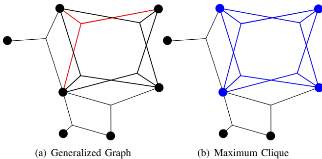
Fig. 1: An example of a generalized consistency graph with edges made of 3-tuples. (a) highlights that each edge denotes consistency of 3 measurements. (b) highlights the maximum clique of the generalized graph in blue.
