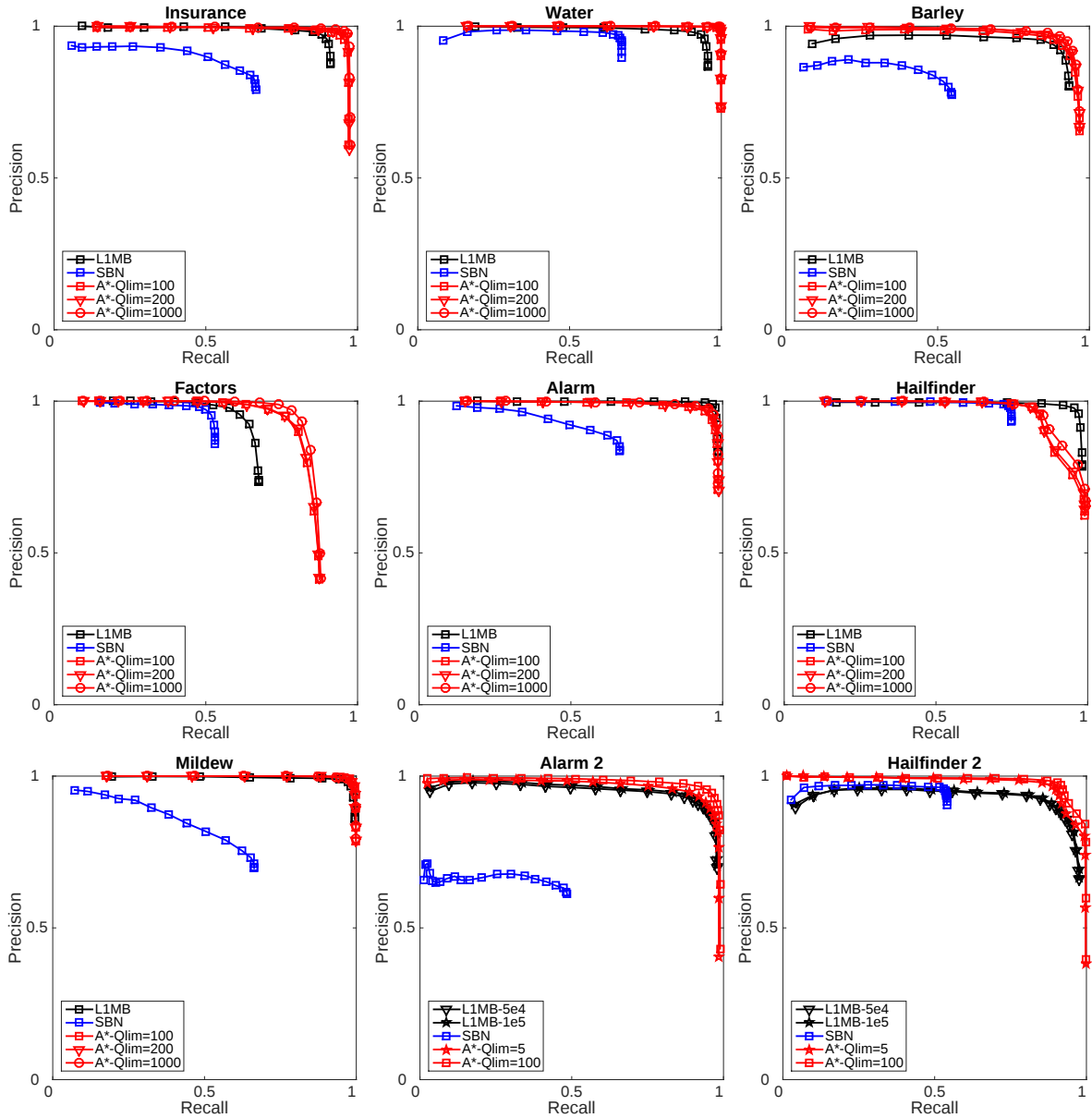
Figure 2.6: Precision/recall curves for the recovery of skeletons of the network structure of benchmark Bayesian networks.
