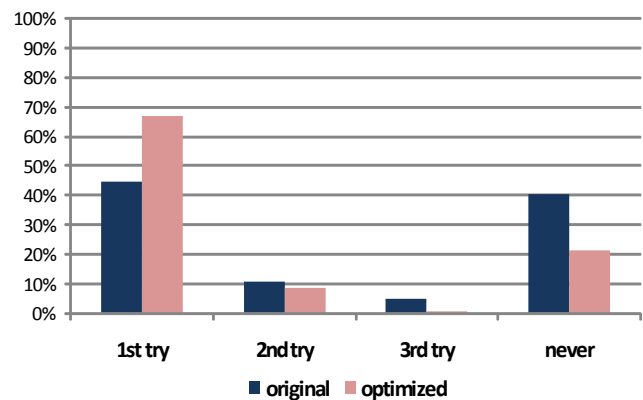
Figure 8. The percentage of CAPTCHAs answered correctly by blind participants using the original and optimized interfaces. The optimized interface enabled participants to answer 59% more CAPTCHAs correctly on their first try as compared to the original interface.
