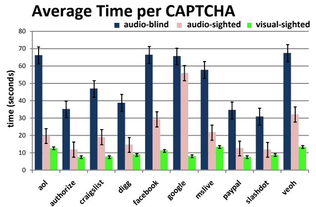
Figure 5. The average time spent by blind and sighted users to submit their first solution to the ten audio CAPTCHAs presented to them. Error bars represent \pm 1 standard error (SE).
