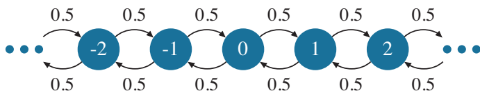
Figure 26.18 Brownian motion.
