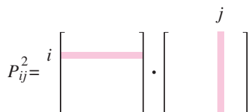
Figure 24.5 (\mathbf{P}^2)_{ij} .
