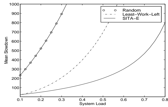
Figure 7: Analytical comparison of mean slowdown on task assignment policies which balance load, as a function of system load.
