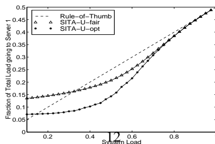
Figure 12: Fraction of the total load which goes to Host 1 under SITA-U-opt and SITA-U-fair and our rule of thumb.
