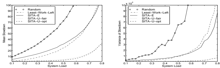
Figure 11: Experimental comparison of mean slowdown and variance of slowdown on all task assignment policies.
