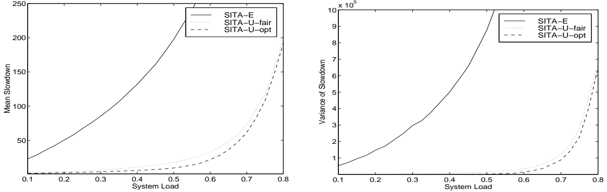
Figure 4: Experimental Comparison of Mean Slowdown and Variance of Slowdown on SITA-E versus SITA-U-fair and SITA-U-opt as a Function of System Load.
