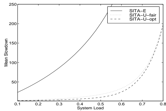
Figure 8: Analytical comparison of mean slowdown for SITA-E and SITA-U-opt and SITA-U-fair, as a function of system load.
