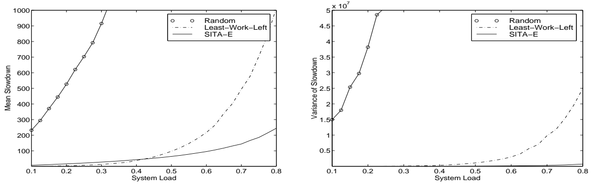
Figure 3: Experimental comparison of task assignment policies which balance load for a system with 4 hosts.
