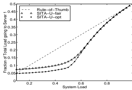
Figure 10: Fraction of the total load which goes to Host 1 under SITA-U-opt and SITA-U-fair and our rule of thumb.
