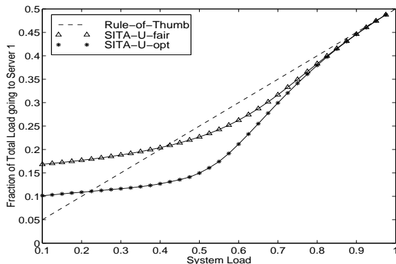
Figure 6: Fraction of the total load which goes to Host 1 under SITA-U-opt and SITA-U-fair and our rule of thumb.
