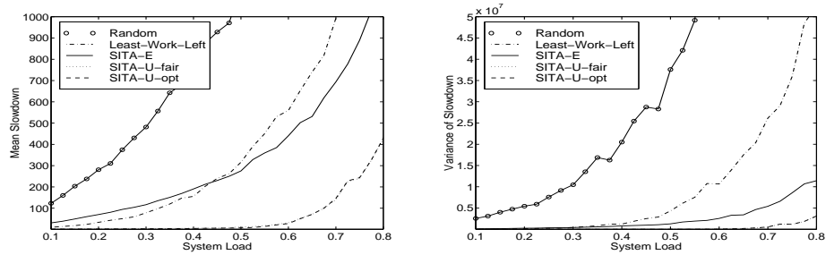
Figure 9: Experimental comparison of mean slowdown and variance of slowdown on all task assignment policies.
