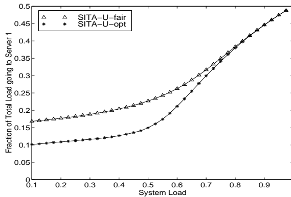
Figure 5: Fraction of the total load which goes to Host 1 under SITA-U-opt and SITA-U-fair.
