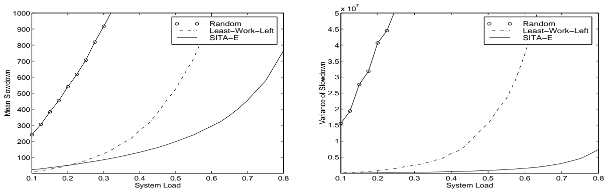
Figure 2: Experimental comparison of task assignment policies which balance load for a system with 2 hosts in terms of: (left) mean slowdown and (right) variance in slowdown.
