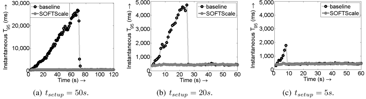
Figure 12: Effect of t_{setup} on instantaneous T_{95} for a 15% \rightarrow 30% jump in load.
