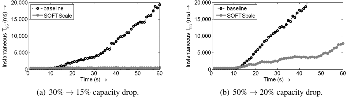
Figure 11: SOFTScale provides significant benefits even when load spikes are caused by a sudden drop in capacity. In the figures above, we drop capacity at the 10s mark.
