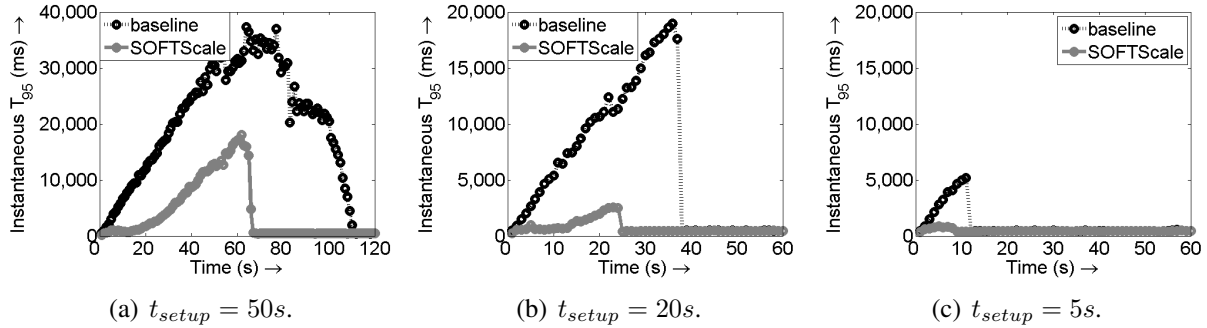
Figure 13: Effect of t_{setup} on instantaneous T_{95} for a 20% \rightarrow 50% jump in load.
