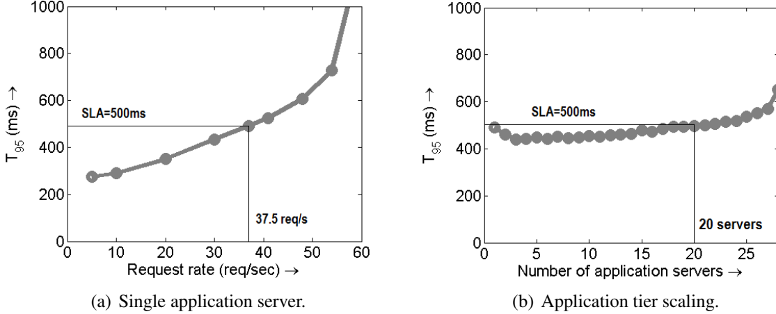
Figure 3: Figure (a) shows that a single application server can handle 37.5 req/s per server. Figure (b) shows that once we have more than 20 application servers, they can no longer handle 37.5 req/s per server because the memcached tier becomes the bottleneck.
