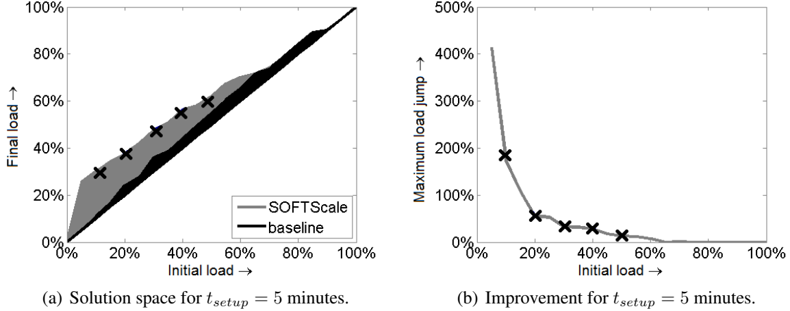
Figure 8: Full range of results for SOFTScale. The crosses in the figures refer to the specific load jump cases shown in Figure 7. Note that SOFTScale’s solution space in Figure (a) is a superset of the baseline’s solution space.
