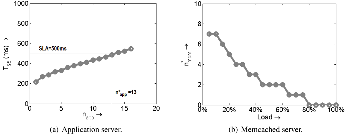
Figure 4: Figure (a) shows that we should invoke SOFTScale whenever the number of requests at the application server exceeds 13. Figure (b) shows n_{mem}^* , the optimal number of application requests that can be simultaneously handled by a memcached server without violating the 500ms SLA, as a function of the total system load.
