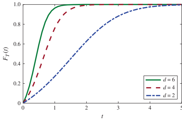
Figure 8. (Color online) \Pr\{T \leq t\} under Redundancy-d when \rho = 0.9 and d = 2, 4 or 6
