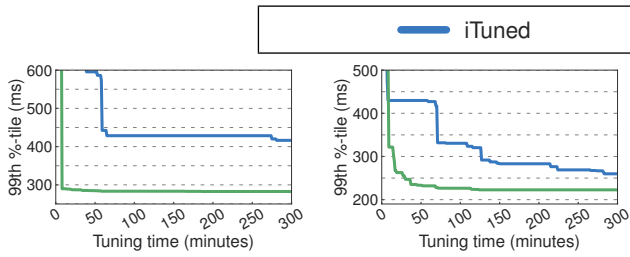
Figure 6: Tuning Evaluation (TPC-C) – A comparison of the OLTP DBMSs for the TPC-C workload when using configurations generated by OtterTune and iTuned.
