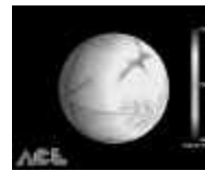
Mantle Convection
