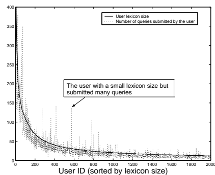
Fig. 6. User lexicon sizes and the number of the queries they submitted in the Vivisimo trace. Solid line plots the sorted user lexicon sizes. Dashed line plots the numbers of the queries submitted by the corresponding users. For scale reasons, this figure is a zoomed in part from a complete figure, but the pattern shown here is general for the complete figure as well.
