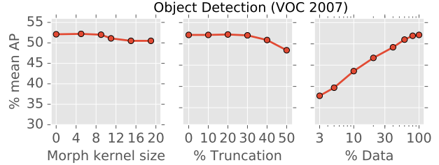
Figure 5. VOC object detection accuracy using our supervised ConvNet as noise is introduced in mask boundaries, the masks are truncated, or the amount of data is reduced. Surprisingly, the representation maintains quality even with large degradation.
