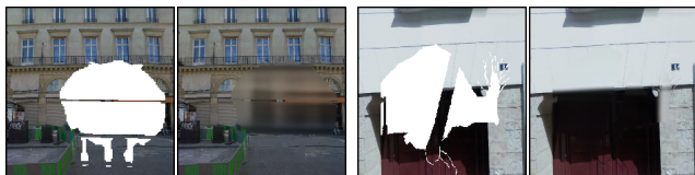
Figure 7: Arbitrary region inpainting for context encoder trained with reconstruction loss on held-out images.
