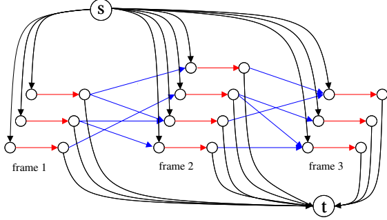
Figure 3. The network model from [25] for three consecutive frames of video. Each space-time location i \in V is represented by a pair of nodes connected by a red edge. Possible transitions between locations are modeled by blue edges. To allow tracks to start and end at any spatiotemporal point in the video, each location i is connected to both a start and termination node. All edges are directed and unit capacity. The costs are c_i for red edges, c_{ij} for blue edges and c_i^s and c_i^t for black edges.
