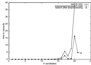
Figure 5: 2 issues, 3 voters, 30 instances per data point.
