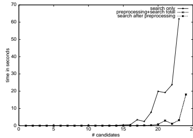
Figure 6: 2 issues, 5 parties, 191 voters, 30 instances per data point.
