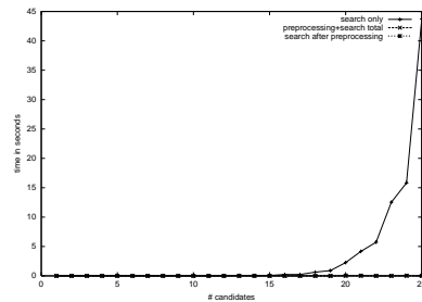
Figure 7: 10 issues, 191 voters, 30 instances per data point.
