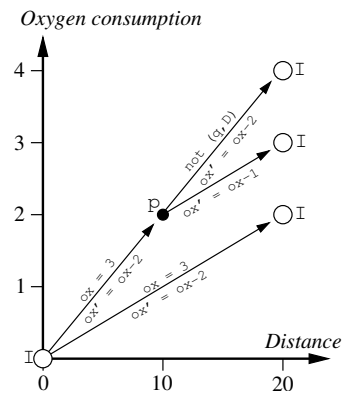
Figure 11: The learned surface task.
