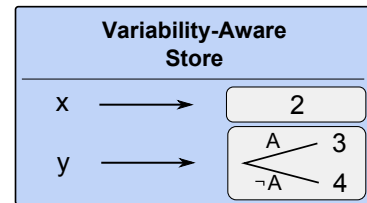
Figure 3.2: Storing conditional values.
