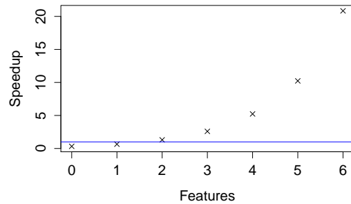
Figure 4.3: Results for early joining benchmark.
