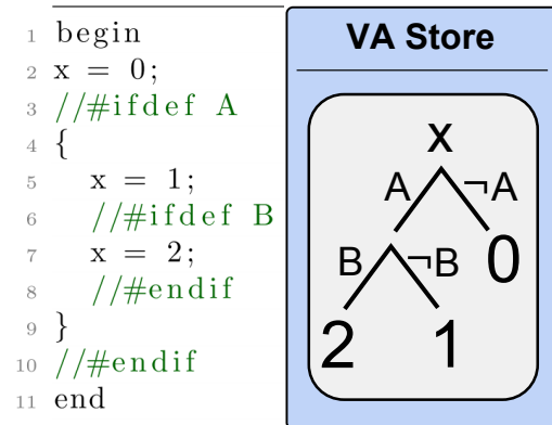
Figure 3.5: Variability propagation in blocks.
