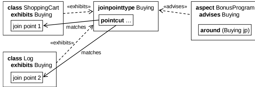
Fig 4. Classes ShoppingCart and Log both depend on the join point type Buying, as does aspect BonusProgram (dashed arrows). The pointcut defined in Buying matches join points in the classes, and is used to trigger the advice in BonusProgram. Note how this corresponds to Fig. 3 (c).
