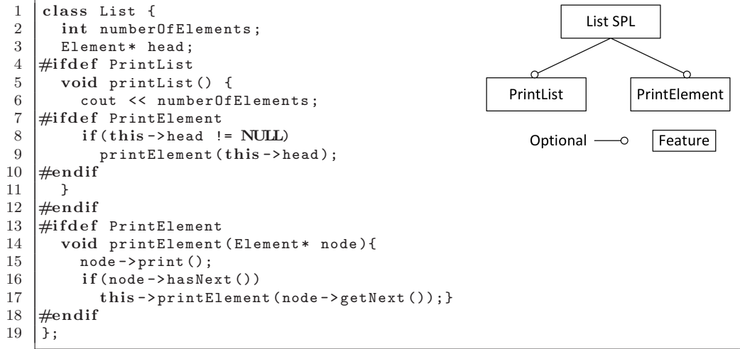
Figure 1: C++ code of a list implementation with two features: PrintList and PrintElement . We show the feature model in the upper right corner.
