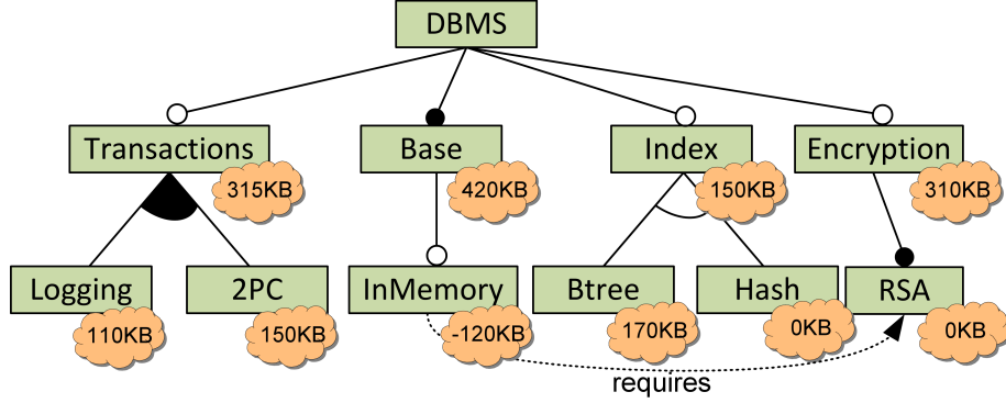
Figure 4: Feature model after approximating the influence of each feature on footprint.
