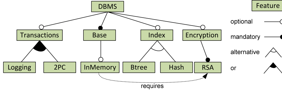
Figure 3: Sample DBMS product line. The root denotes the concept. 2PC: two phase commit protocol.
