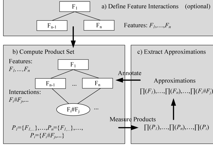
Figure 2: The process of computing approximations of non-functional properties for features and feature interactions.
