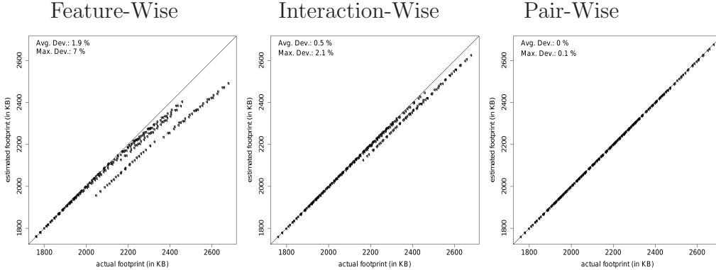
Figure 5: Q-Q plot: Measured and predicted footprint in KB of Berkeley DB (compiled as static link library) using different approaches.
