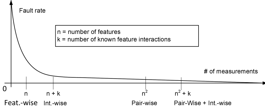
Figure 6: Conceptual relation between number of measurements and fault rate of predictions.
