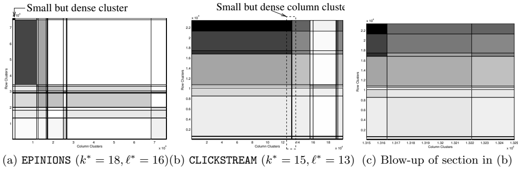
Figure 6: Cross-associations for EPINIONS and CLICKSTREAM. The matrices are organized successfully in homogeneous regions. (c) shows that our method captures dense clusters, irrespective of their size.
