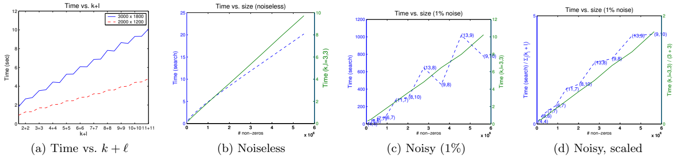
Figure 7: (a) Wall-clock time for one row and column swapping (step (2) and (4)) vs. k + l is linear (shown for two different matrix sizes, with n_1(D) = 0.37n(D) ). (b,c) Wall-clock time vs. number of non-zeros, for CrossAssociationSearch (dashed) and for ReGroup with (k, l) = (3, 3) (solid). The stopping values (k^*, l^*) are shown on plots (c,d), if different from (3, 3) . (d) Wall-clock times of plot (c), scaled by \propto 1/(k^* + l^*)^2 .
