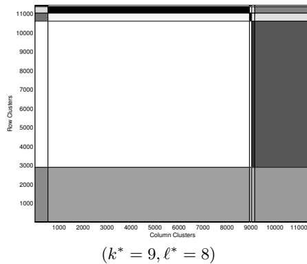
Figure 8: Cross-associations for OREGON.
