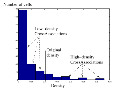
Figure 10: The algorithm splits the original CLASSIC matrix into homogeneous, high and low density Cross-associations.
