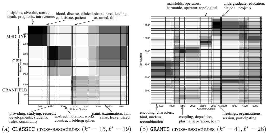
Figure 5: Cross-associations for CLASSIC and GRANTS: Due to the dataset sizes, we show the Cross-associations via shading; darker shades correspond denser blocks (more ones). We also show the most frequently occurring words for several of the word (column) groups.
