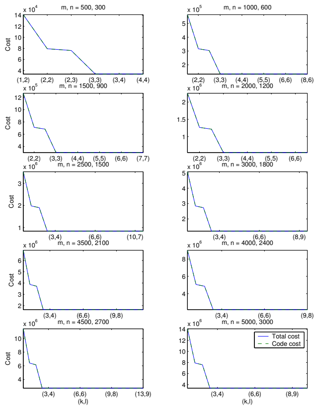
Figure 11: Progression of cost during search on synthetic cave graphs (for varying sizes); see also Figure 7(b).
