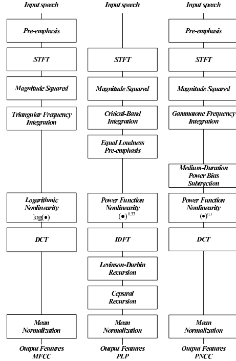
Figure 1: Comparison of the PNCC feature extraction discussed in this paper with MFCC and PLP feature extraction.
