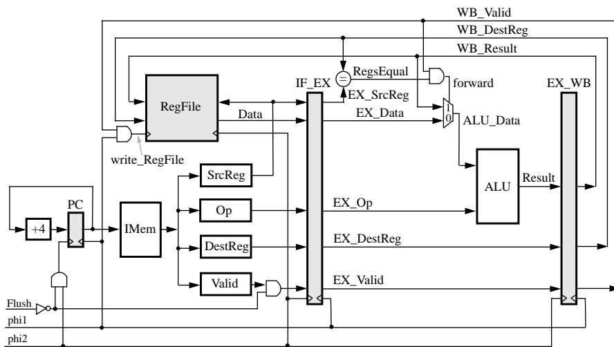
Fig. 1. Block diagram of a 3-stage pipelined processor.
