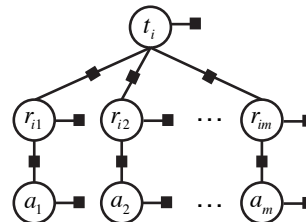
Figure 2: A factor graph representation of the within-event model, relating the event type t_i of trigger candidate i to the role type r_{ij} of each argument candidate j along with its entity type a_j .
