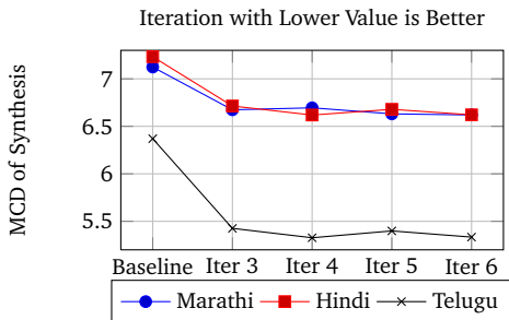
Figure 3: Objective Improvements using Iterative Targeted Acoustic Models
