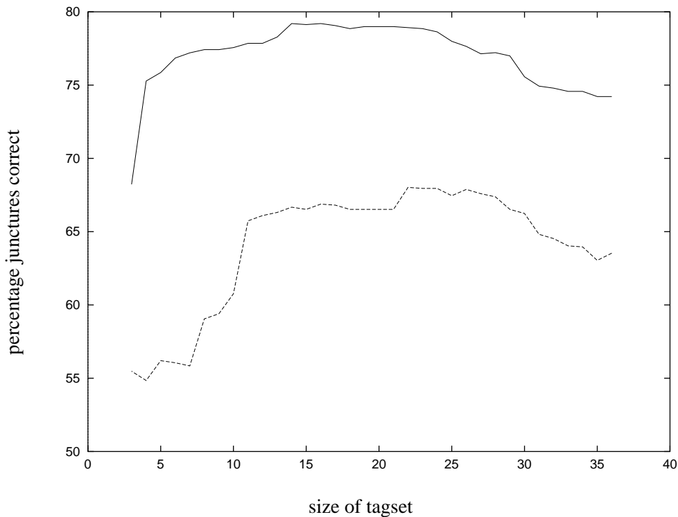
Figure 2: Plot of junctures-correct for a 6-gram (upper line) and 1-gram (lower line) against K , the size of the tagset.
