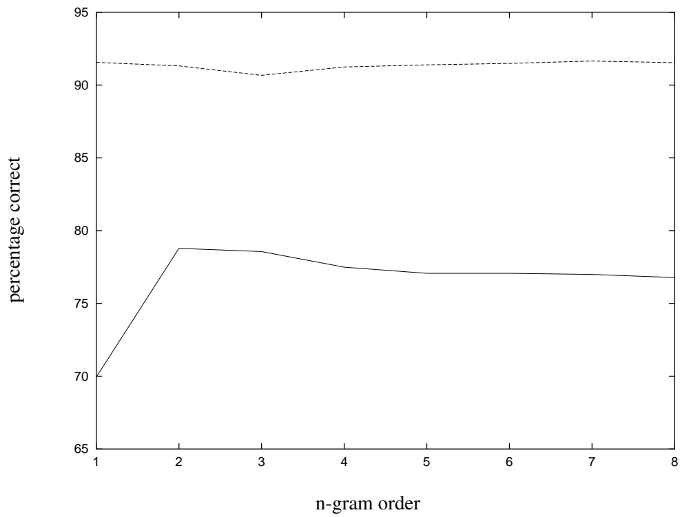
Figure 5: Plot of junctures-correct (upper line) and breaks-correct (lower line) against order of n-gram
