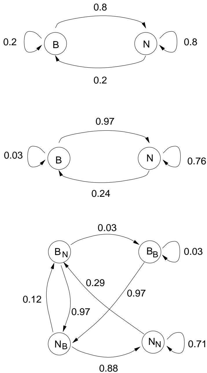
Figure 1: Models for N=1 , N=2 and N=3 , showing actual transition probabilities calculated from the training data. The states marked B are for breaks and those marked N are for non-breaks. Subscripts in state names indicate the juncture type of the previous state. In the N=1 case the transition probabilities are just the context independent probabilities of the juncture types occurring, i.e the transition probabilities to a state don't depend on the previous state. In the N=2 case, the transition probabilities take into account the previous juncture. Thus in this model it is very unlikely that a break will follow a break (0.03), while in the N=1 case this would still have a relatively high probability (0.2). Looking at the probabilities of sequences of non-breaks, we see differences in the probability of a non-break following two previous non-breaks. As N increases, we see that the probability of long sequences of non-breaks decreases ( P(N_i|P_{i-1}, P_{i-2}) = 0.8 for N=1 , 0.76 for N=2 and 0.71 as N=3 ). Thus a higher order ngram helps prevent unrealistically long sequences of just non-breaks or just breaks. The POS sequence model probabilities (not shown here) are associated with each state. All states of the same basic type are the same and so the probability distributions for state B_B (a break following a break) are the same as for state B_N (a break following a non-break).
