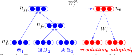
Figure 3: The structure generation procedure of the source sub-phrase “所 通过 决议” and the structure reconstruction procedure of the target sub-phrase “resolution adopted”. According to word alignments (“2-1 3-0”), the node n_{\bar{f}_1} and n_{\bar{f}_2} are SAC ones while the node n_{\bar{f}_3} is a non-SAC node.
