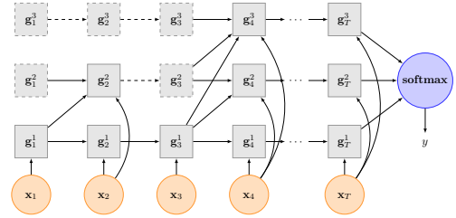
(b) Unfolded MT-LSTM with Fast-to-Slow Feedback Strategy
