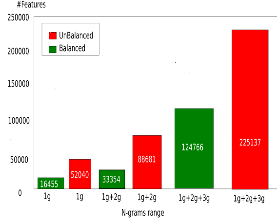
Figure 3: Feature Counts. Number of unigram, bigram, and trigram features per each class category.
