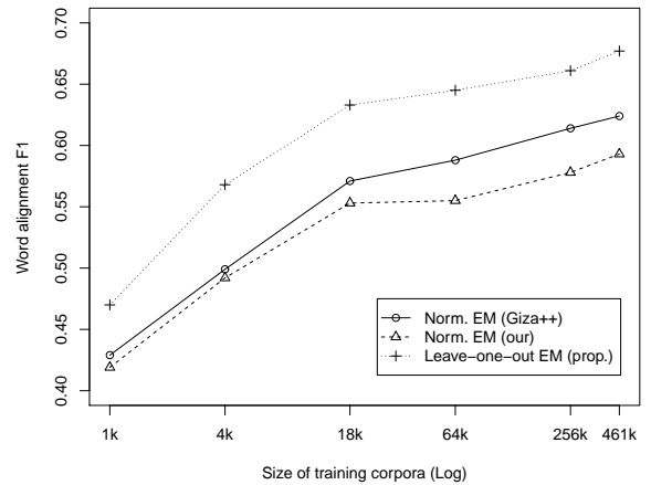
Figure 2: Curve of word alignment accuracy (F 1 ) under training corpora of different sizes.
