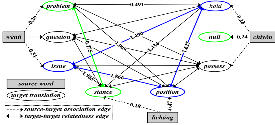
Figure 2: Translation graph of the example shown in Figure 1. Relatedness scores on edges are shown for two group of translations \{“problem”, null, “stance”\} ( green ) and \{“issue”, “hold”, “position”\} ( blue ), which are estimated with PMI. Note that the null node does not have any relations with other nodes. Besides, two translation combinations \{“problem”, null, “stance”\} (green) and \{“issue”, “hold”, “position”\} (blue) have different strengths of relatedness.
