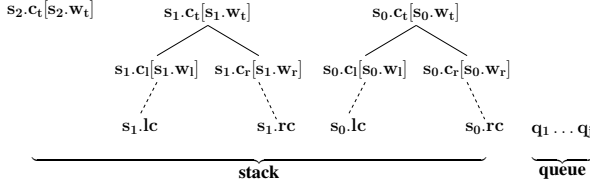
Figure 2: Features available for scoring. s_x denote a position in the stack. Stack positions are local trees of depth 1, features can access its top , left and right nodes. The suffixes c p , w p , lc , rc denote respectively the delexicalized category, the head token, the left corner token, the right corner token of a stack position. For tokens elements accessible from the stack ( s_x.w_x ) and from the queue ( q_x ), features can access the word form, pos tag or any morphological feature m available for that language as described in the table at the right
