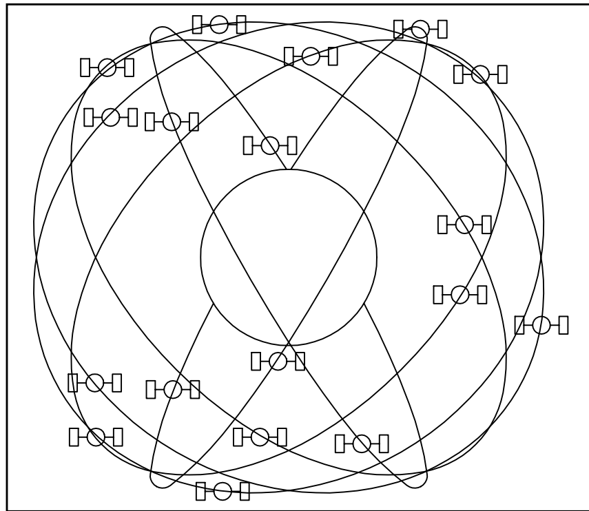
Figure 29 Orbital Configuration
