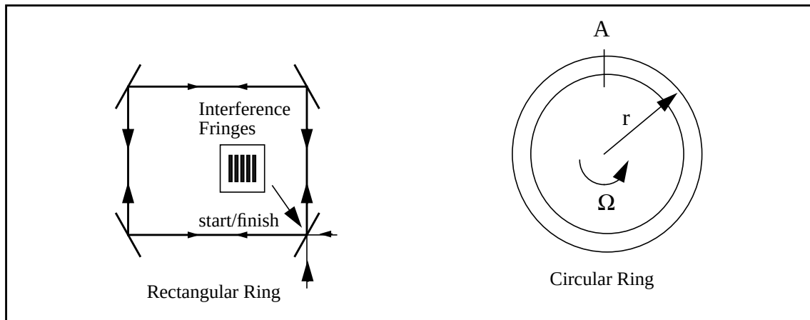
Figure 12 Ring Interferometer
