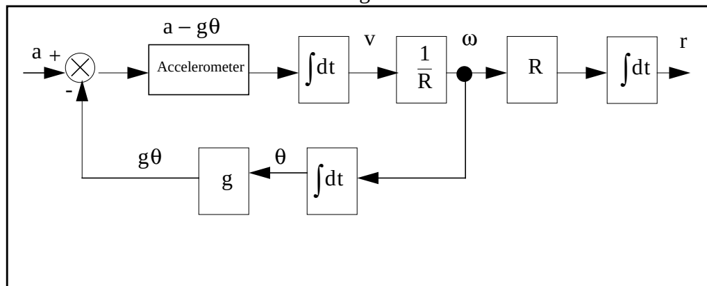
Figure 19 Schuler Loop
