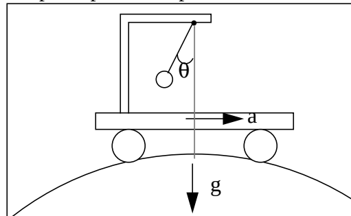
Figure 18 Accelerated Pendulum
