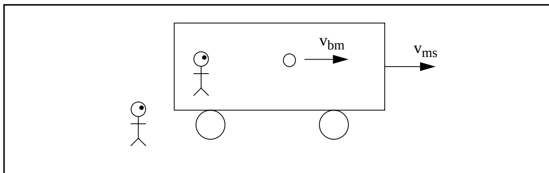
Figure 1 Einstein's Train
