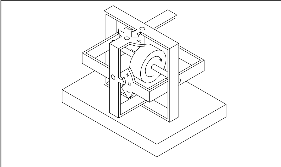
Figure 8 Mechanical Gyroscope
