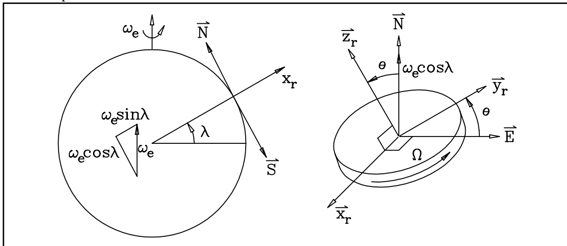
Figure 11 Gyrocompass
