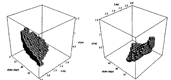
Fig. 12 Two views of set of feasible plans that meet all constraints given scenario in Fig. 9 and also sweep a volume of soil that is greater than 90% of the volume of the bucket.
