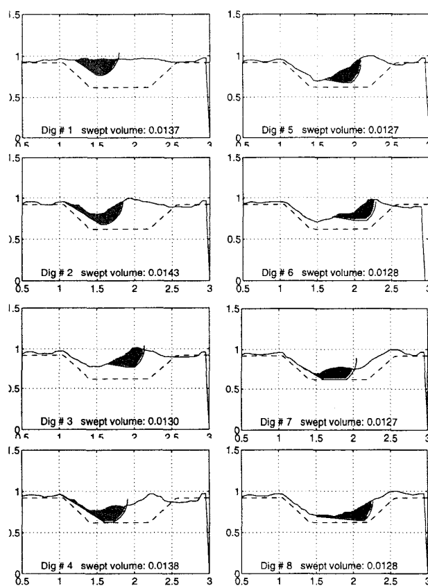
Fig. 15 The first eight steps in the creation of a trench. The desired trench is shown by the dashed line. The shaded region is the volume of soil (in m3) estimated to be swept by the excavator bucket.
