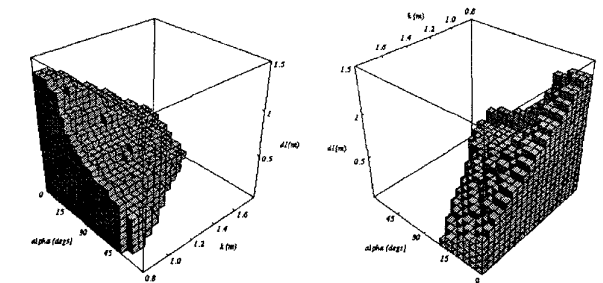
Fig. 11 Two views of set of feasible plans that meet the force constraints given scenario in Fig. 9.
