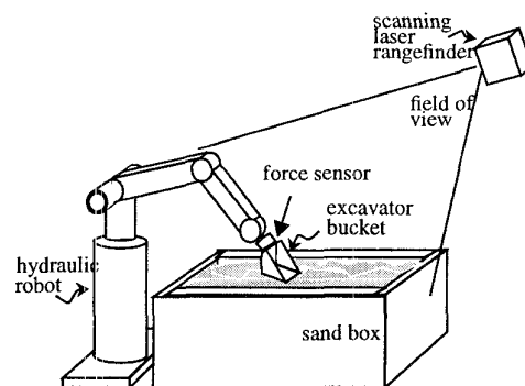
Fig. 13 Testbed
