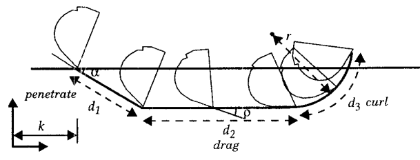
Fig. 8 A typical dig during a trenching operation. There are typically three distinct types of motion— penetrate , drag and curl . A digging trajectory of this form can be represented by a seven-tuple (k, \alpha, d_1, d_2, d_3, r, \rho) .
