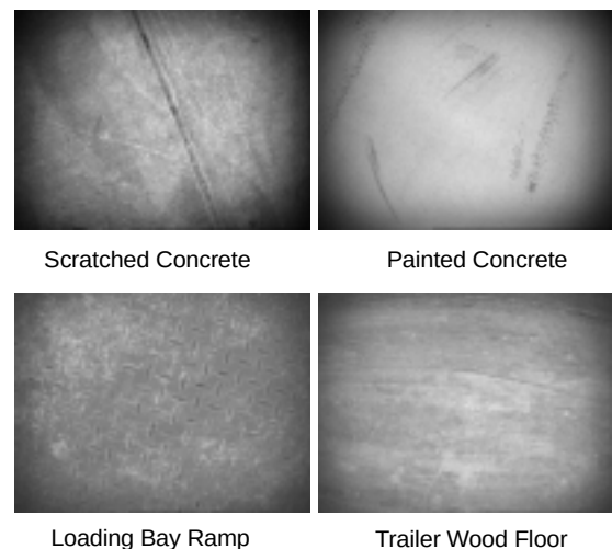
Figure 4: MANUFACTURING PLANT FLOOR IMAGERY. Many man made surfaces exhibit locally unique texture.
