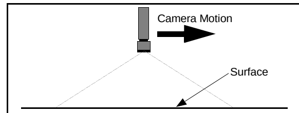
Figure 1: SIMPLEST SCENARIO: Here a camera is erected normal and at constant height with respect to a surface. It moves parallel to the surface - hence variations in foreshortening do not occur.
