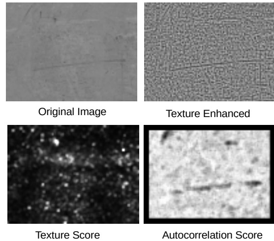
Figure 5: ANALYSIS OF TYPICAL FLOOR IMAGE. While it may subjectively seem that this concrete floor image lacks sufficient texture, it is actually acceptable at every single pixel.
