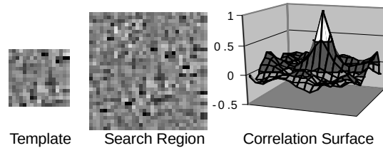
Figure 3: PRINCIPLE OF OPERATION. The translational pose error can be found as the position of the peak in a surface: the correlation as a function of disparity.
