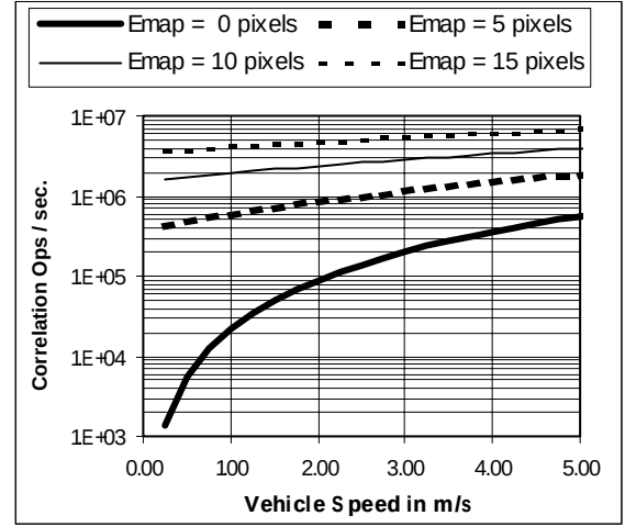
Figure 8: PROCESSING REQUIREMENTS. Increase with vehicle speed. From bottom to top, the 4 curves are for \epsilon_{MAP} of 0, 5, 10, and 15, pixels of size 2.5 mm.
