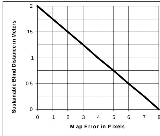
Figure 10: SUSTAINABLE EXCURSION OVER UNKNOWN REGION. For a search radius of 8 pixels, a pixel size of 2.5 mm, and a map error of 2 pixels, 1.5 meters of excursion over unknown, unmapped, or changed surface can be accommodated.
