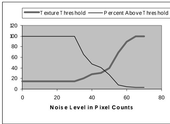
Figure 6: NOISE IMMUNITY. For a maximum grey level value of 255, it takes random noise with a standard deviation of 60 counts before the highest texture regions in the image generate false positives.
