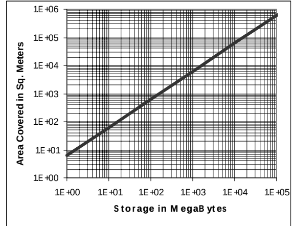
Figure 7: STORAGE REQUIREMENTS. Up to 10 Km of guideway can be stored at 1 mm resolution in 1 GByte of memory.
